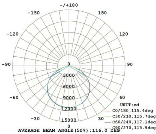
200W Light distribution curve
