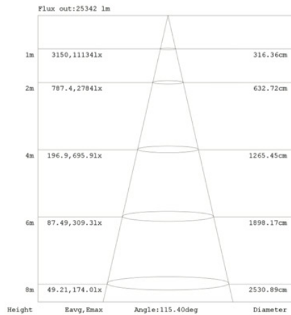
200W Average Illumination
